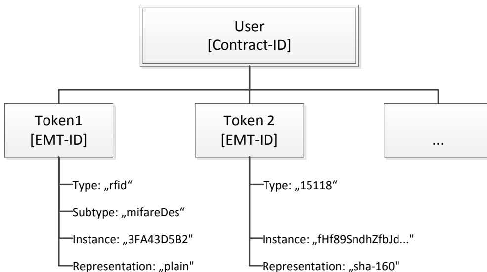
Figure 11: ID-Structure
